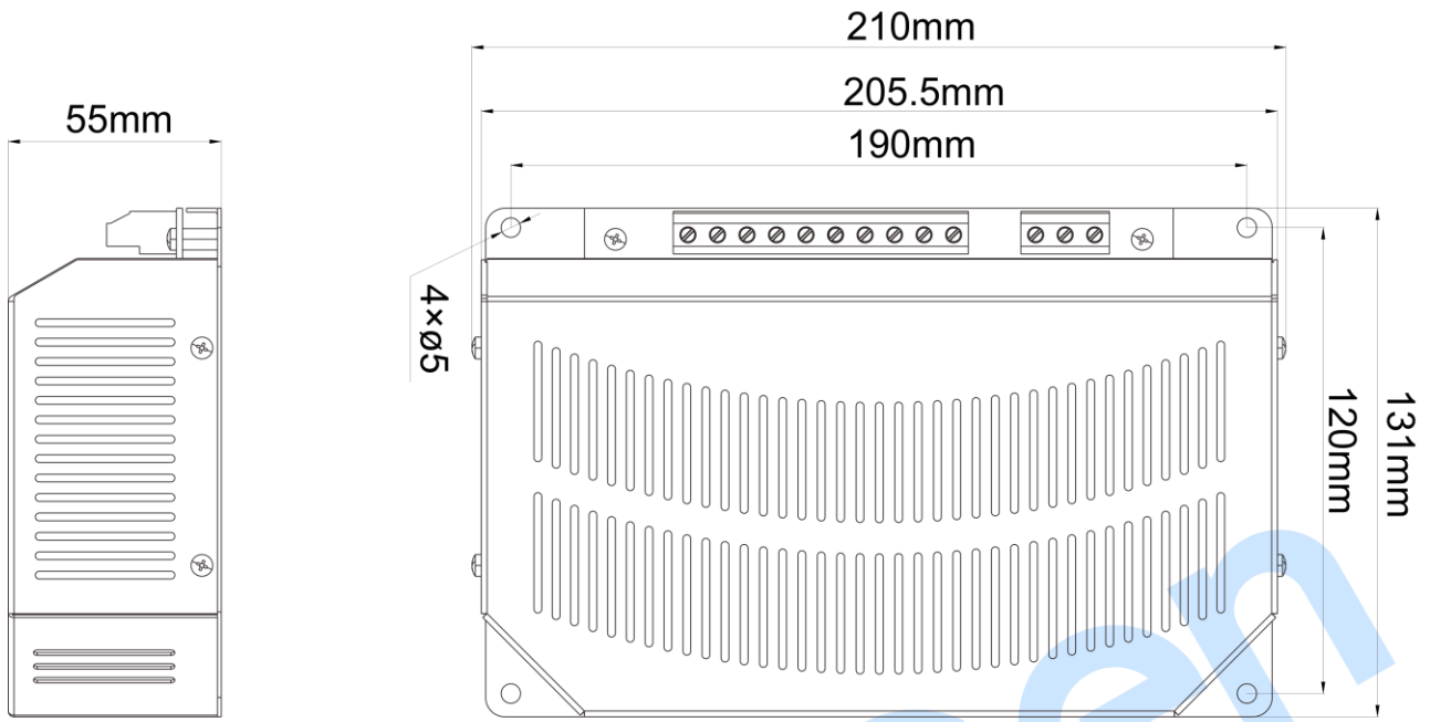
Fig.5 BAC2410BST Case Dimension
