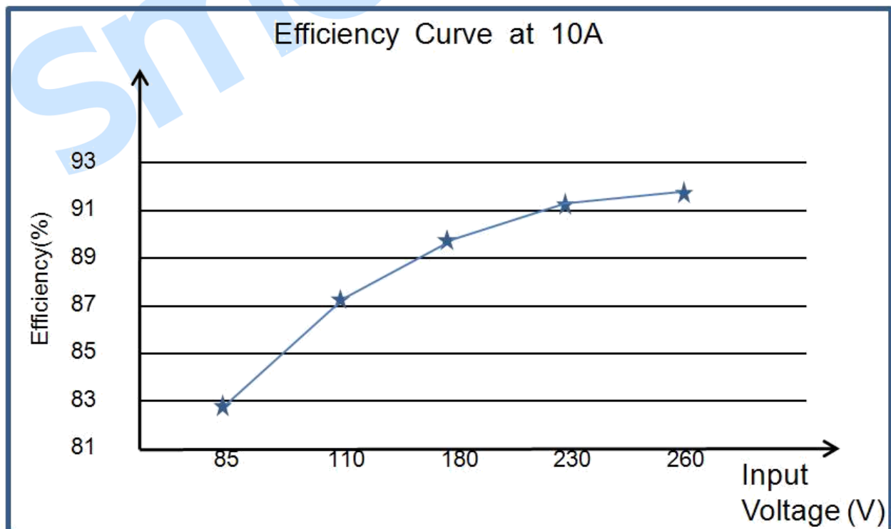
Fig.3 Efficiency Curve
