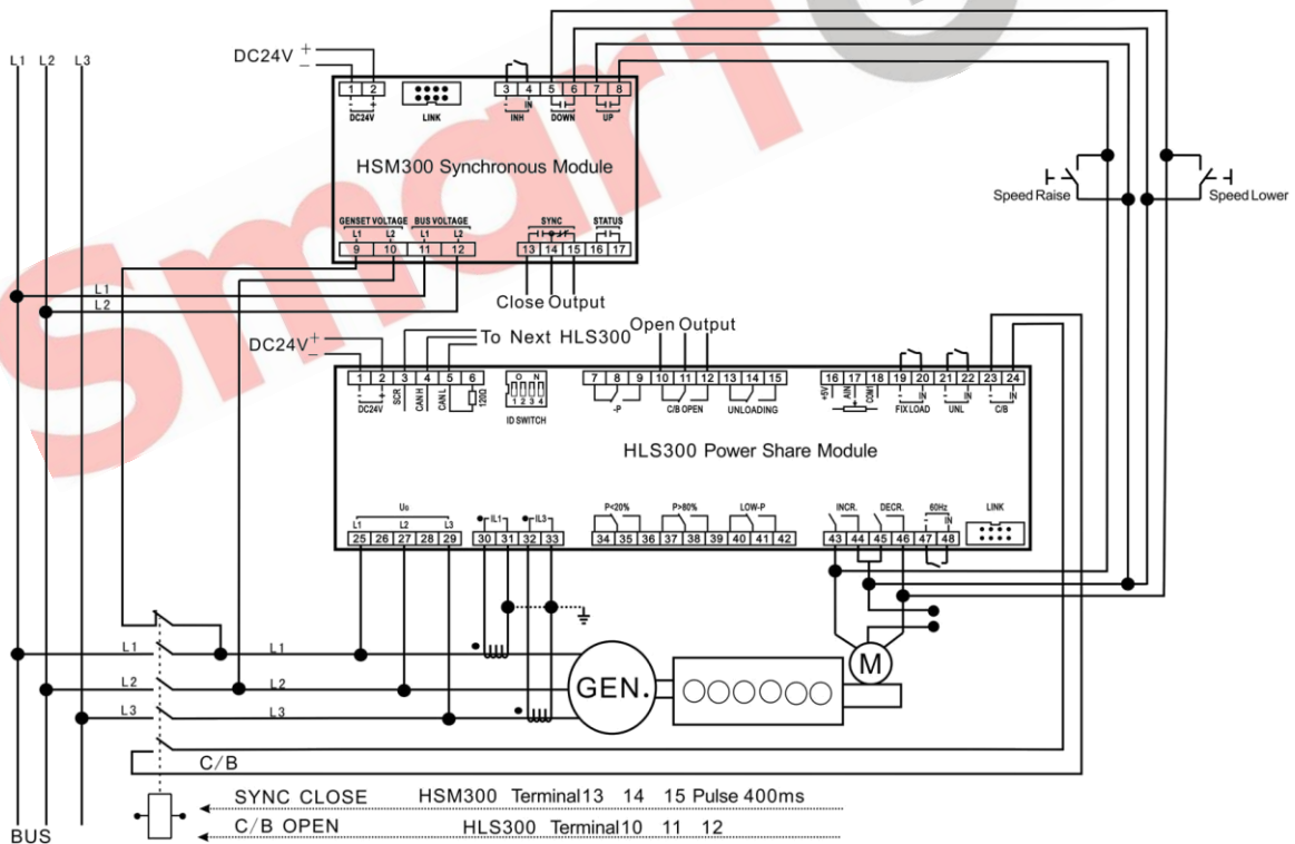
Fig.5 - HSM300-HLS300 3Phase 3Wire Typical Application
