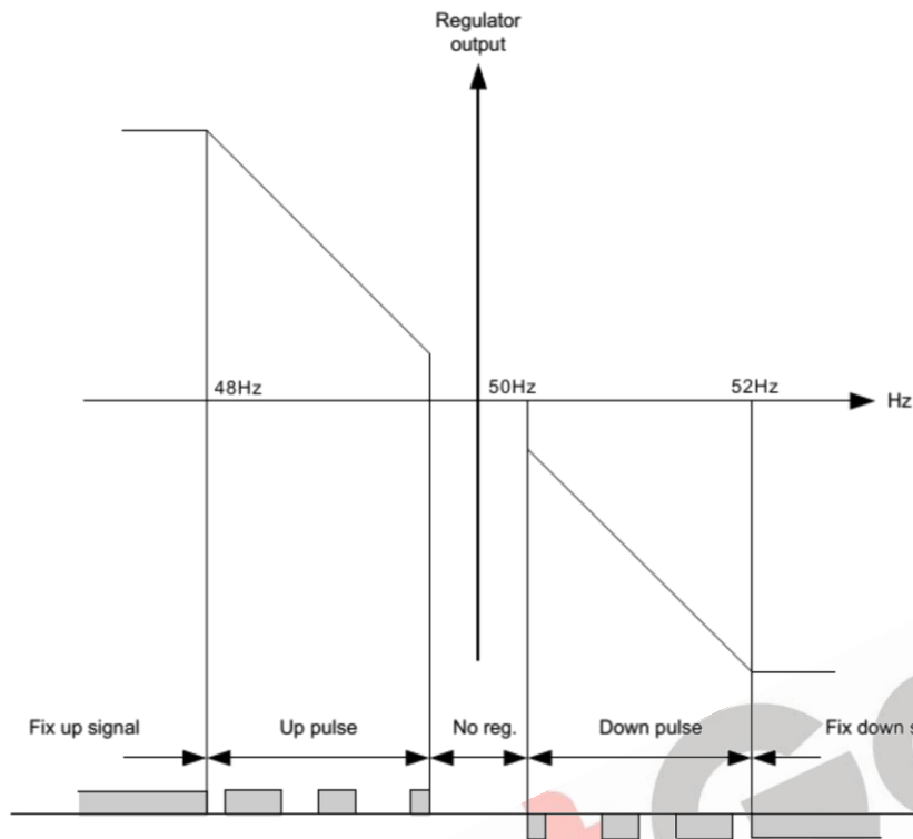
Fig.3 - working principle of raise/drop speed relay
